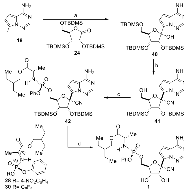
Scheme 9
