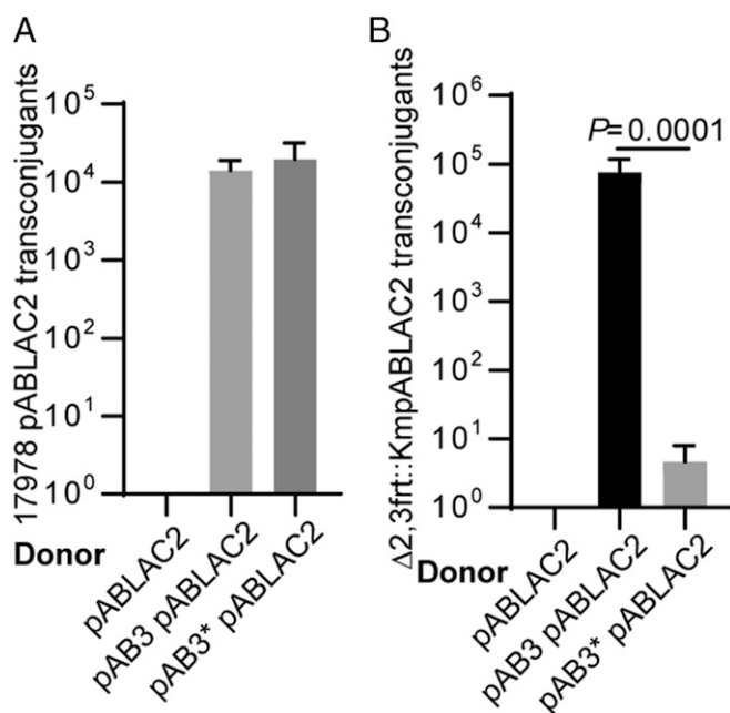
Fig. 3. LCP-mediated SMP mobilization. Data are mean \pm SD; n = 3 independent replicates. Conjugation assays are at a donor:recipient ratio of 5:1. Quantification of recovered pABLAC2 transconjugants (indicated on the left of each panel); donor strains are indicated in the x axis. (A) pABLAC2 conjugation is nondetectable if pAB3 is not present in the donor strain. (B) pABLAC2 efficiency of conjugation to a T6SS-mediated killing susceptible recipient strain is highly reduced in the presence of an LCP unable to repress T6SS. Statistical analysis was performed using one-way ANOVA and the Tukey–Kramer multiple-comparison test.
