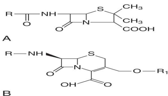
Figure 2. General Structures of (I) Penicillins and (II) Cephalosporins.
