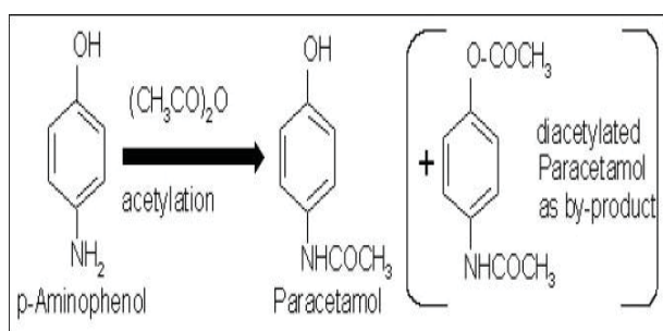
Figure 1. Production of Paracetamol from intermediate, p-Aminophenol. [15]
