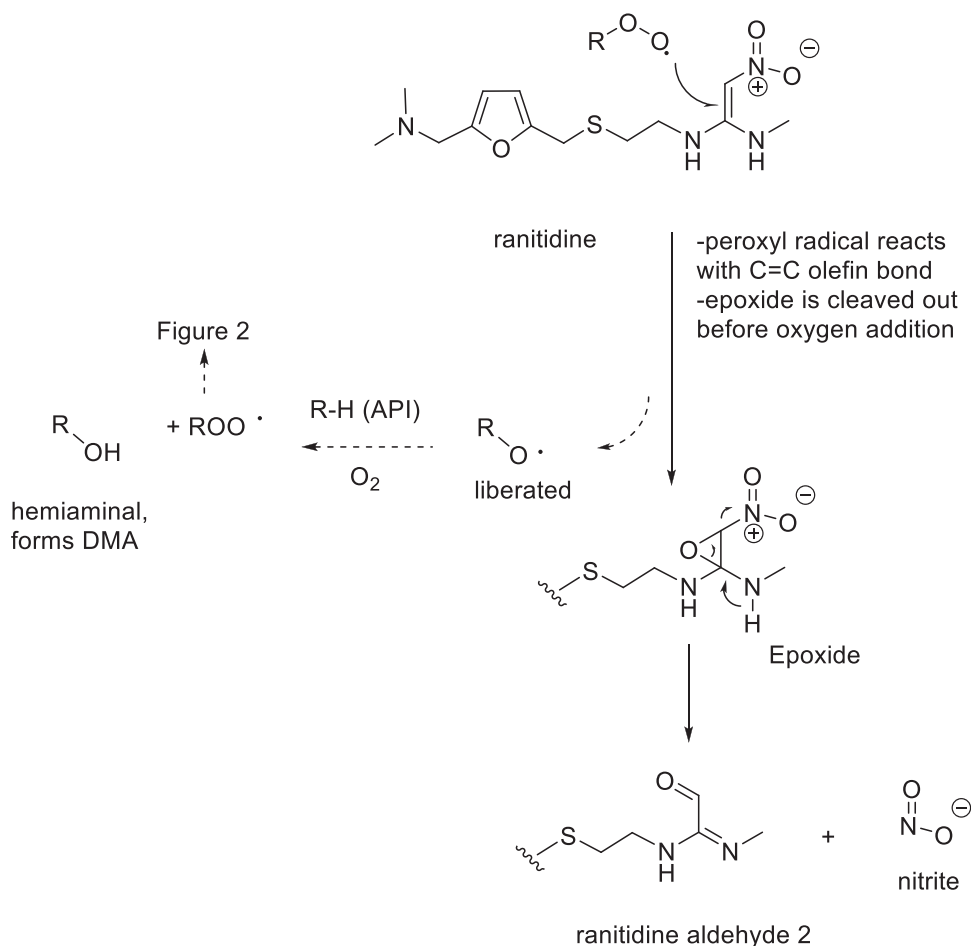
Figure 3. Reaction of peroxy radical with the C=C olefin bond of ranitidine. Shown is olefin epoxidation. Either amine N-H bond can facilitate the epoxide rearrangement to an aldehyde with liberation of nitrite; we show the N-methyl amine case above. Note consumption of oxygen.
